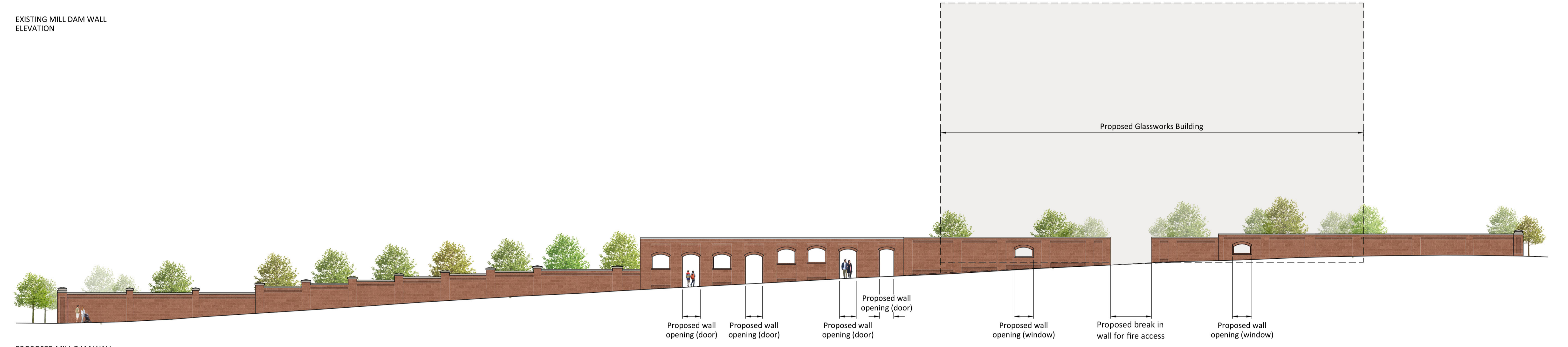
PROPOSED MILL DAM WALL ELEVATION
